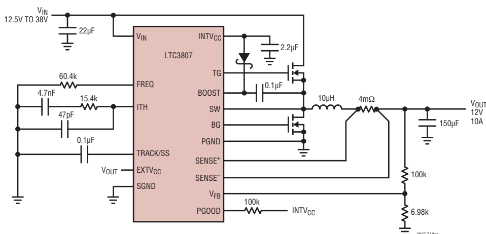
High Efficiency 12V/10A Step-Down Converter
